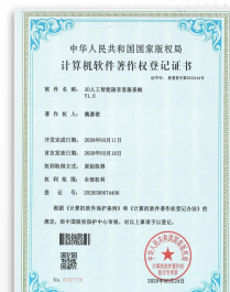
Software Patents
